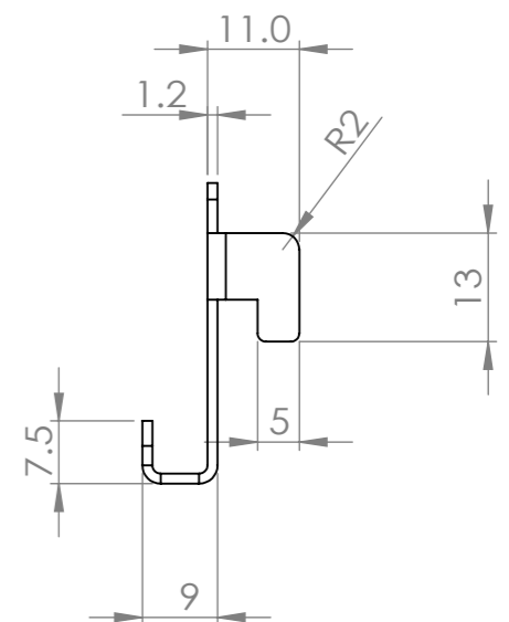
DETAIL V SCALE 1 : 1
