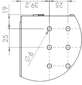
DETAIL P SCALE 1 : 2
