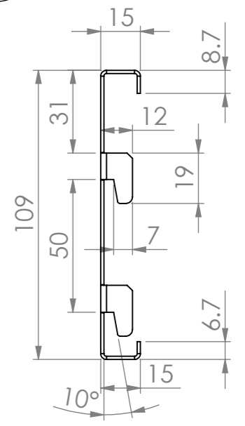
DETAIL D SCALE 1 : 2
