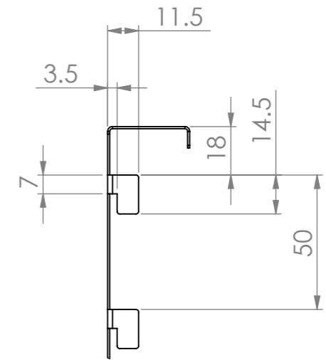
DETAIL Q SCALE 1 : 2
