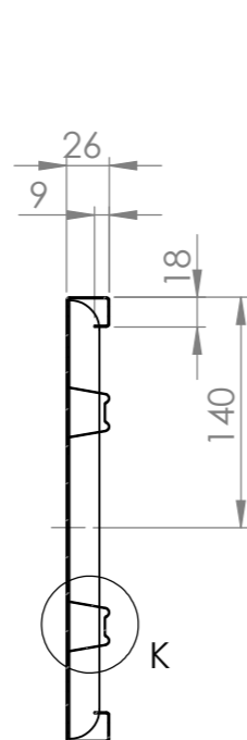
SECTION J-J
