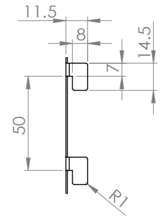
DETAIL M SCALE 1 : 2
