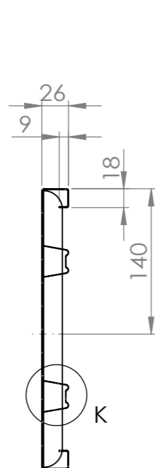
SECTION J-J
