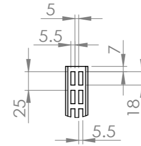
DETAIL G SCALE 1 : 5
